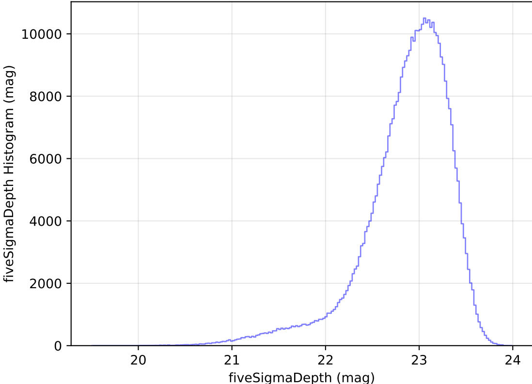
too_elab_heavy_r64_d3_griz_v3.4_10yrs WFD z band: fiveSigmaDepth Histogram
