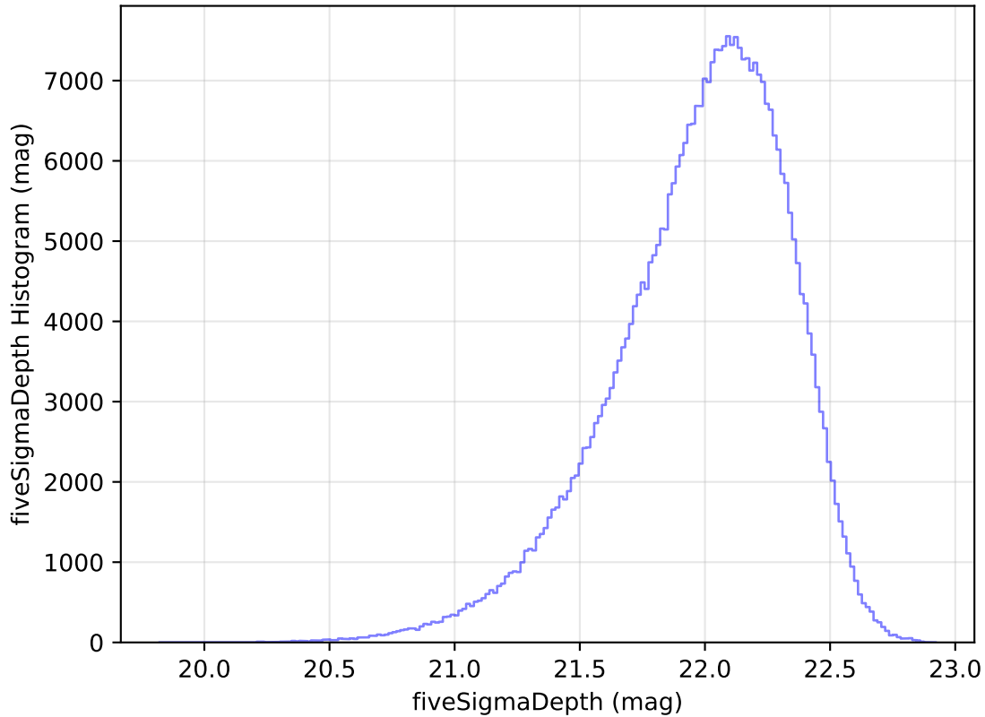
too_elab_heavy_r64_d3_griz_v3.4_10yrs WFD y band: fiveSigmaDepth Histogram
