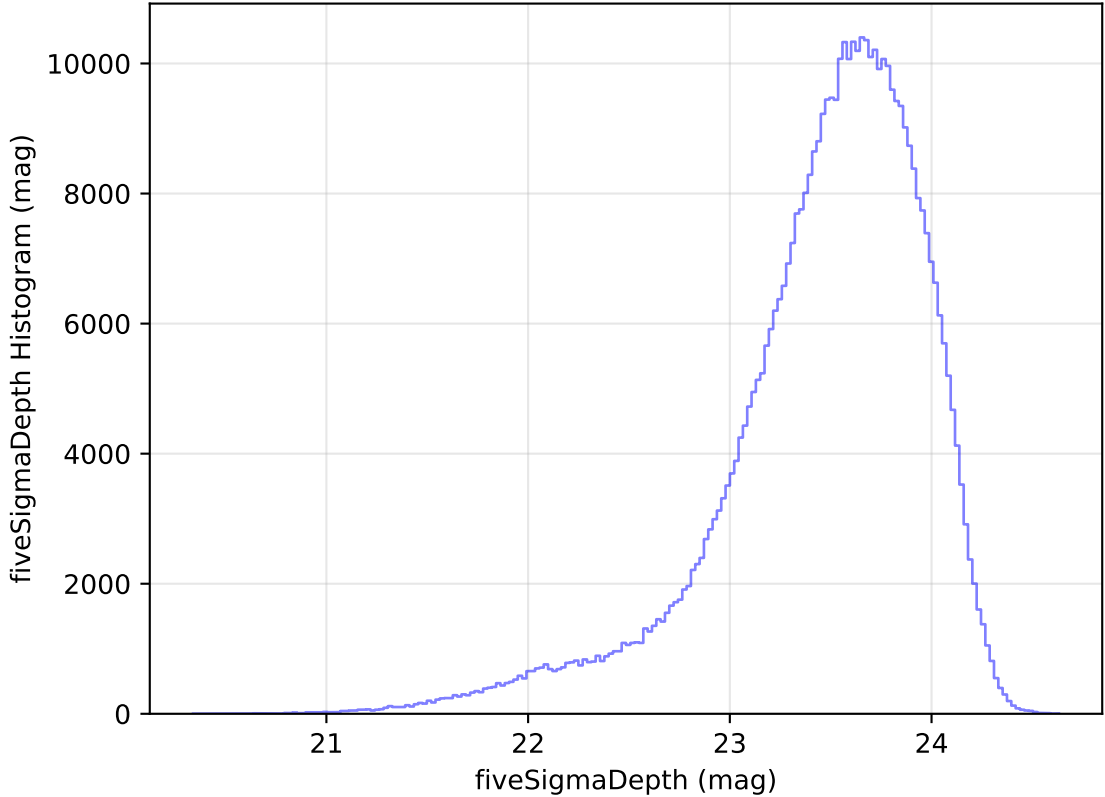
too_elab_heavy_r64_d3_griz_v3.4_10yrs WFD i band: fiveSigmaDepth Histogram
