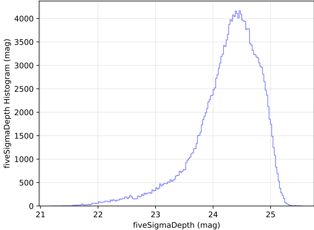
too_elab_heavy_r64_d3_griz_v3.4_10yrs WFD g band: fiveSigmaDepth Histogram
