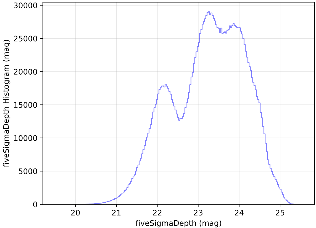
too_elab_heavy_r64_d3_griz_v3.4_10yrs WFD all bands: fiveSigmaDepth Histogram
