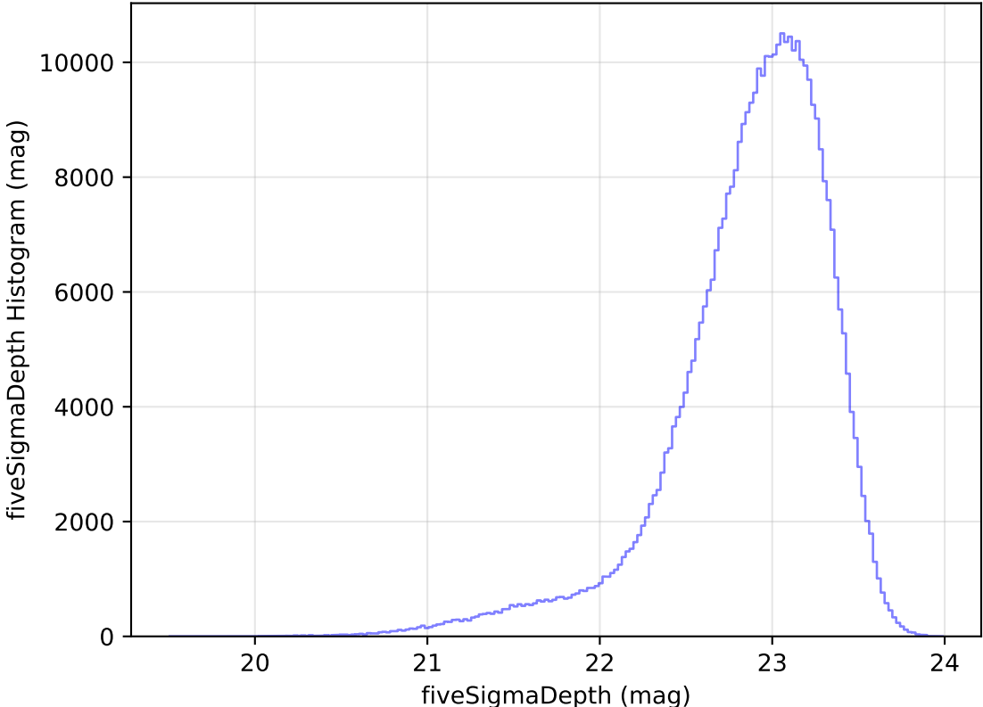
too_elab_heavy_r64_d3_griz_v3.4_10yrs All sky z band: fiveSigmaDepth Histogram
