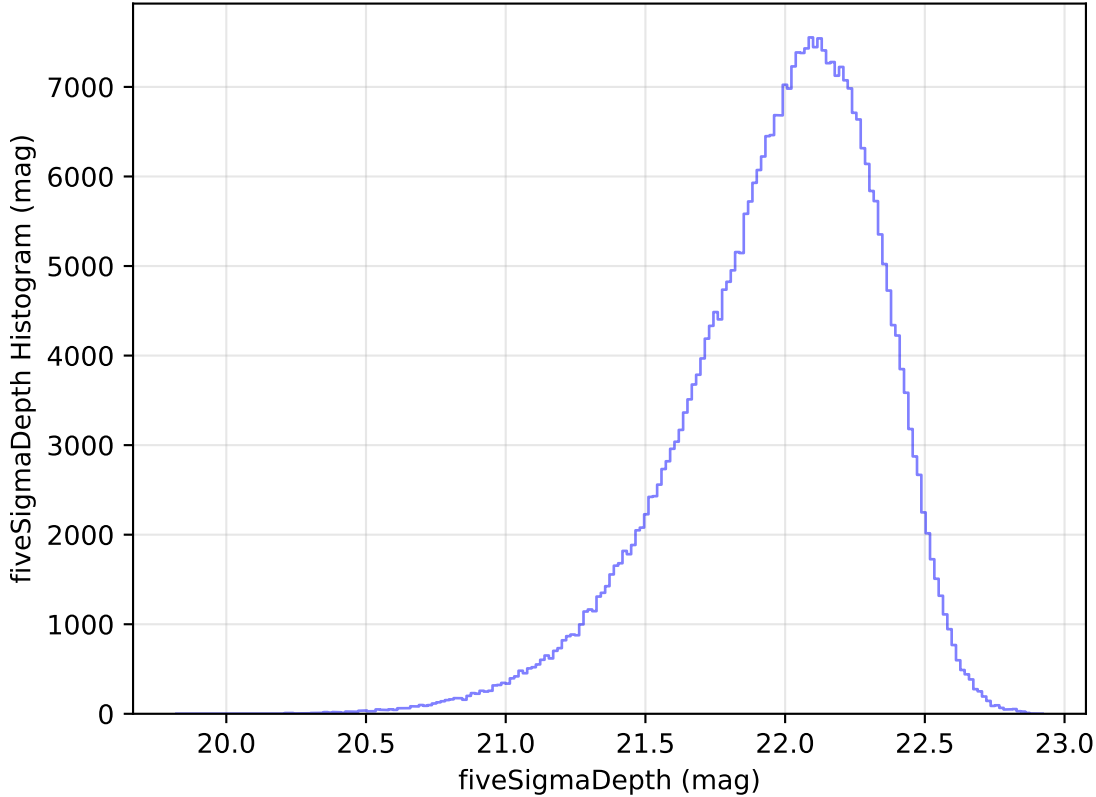
too_elab_heavy_r64_d3_griz_v3.4_10yrs All sky y band: fiveSigmaDepth Histogram
