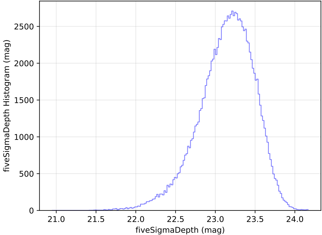
too_elab_heavy_r64_d3_griz_v3.4_10yrs All sky u band: fiveSigmaDepth Histogram
