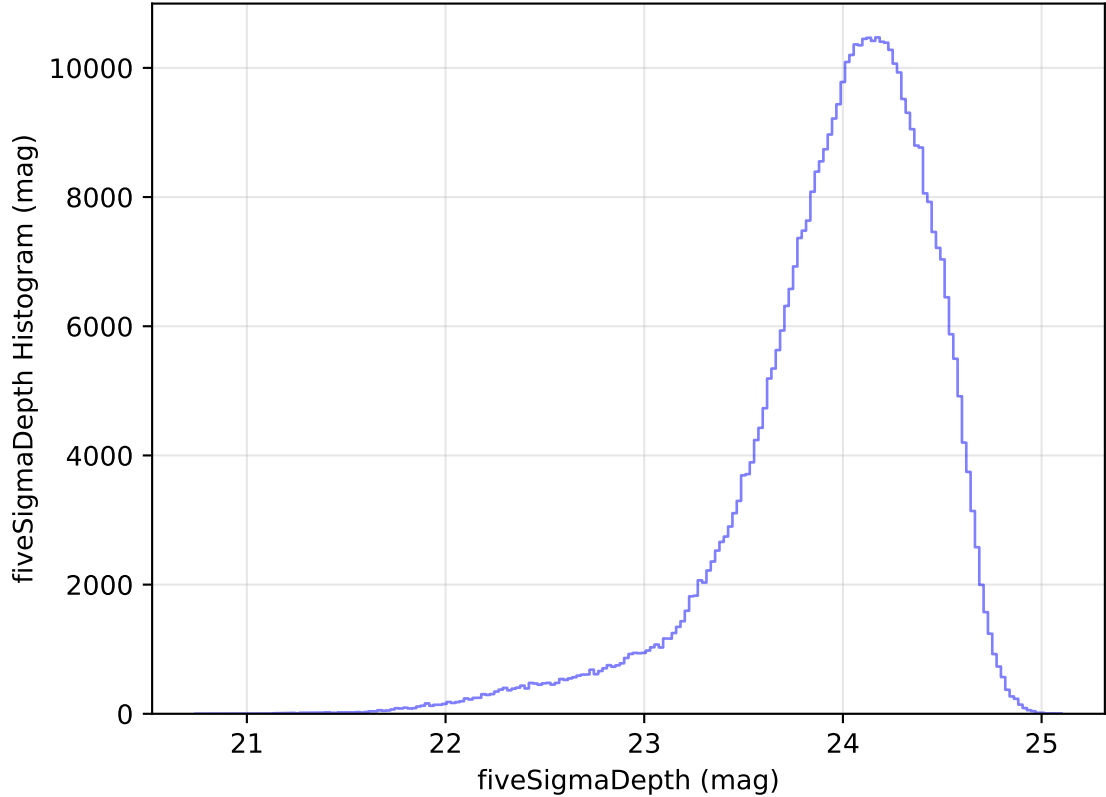
too_elab_heavy_r64_d3_griz_v3.4_10yrs All sky r band: fiveSigmaDepth Histogram
