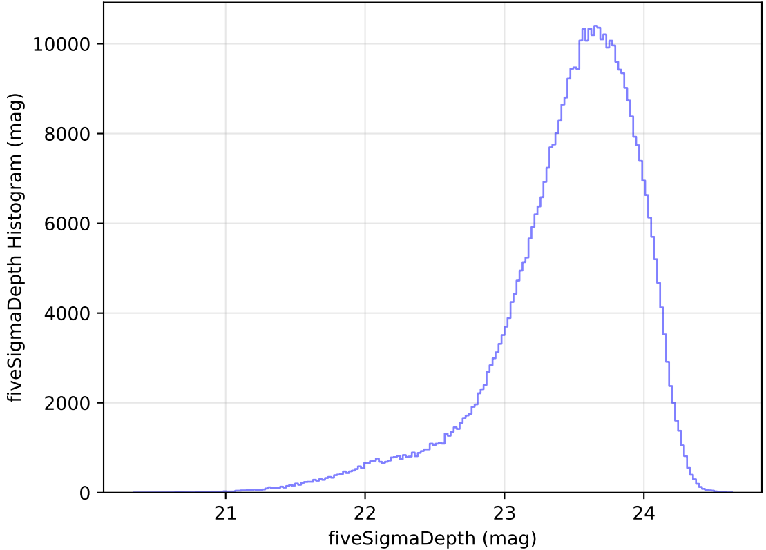
too_elab_heavy_r64_d3_griz_v3.4_10yrs All sky i band: fiveSigmaDepth Histogram
