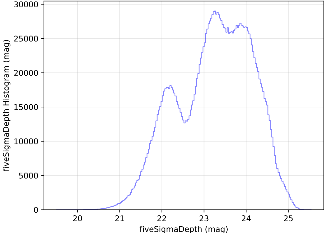
too_elab_heavy_r64_d3_griz_v3.4_10yrs All sky all bands: fiveSigmaDepth Histogram
