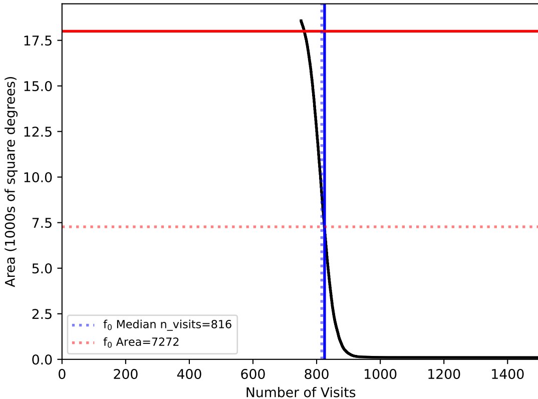
too_elab_heavy_r64_d3_griz_v3.4_10yrs WFD: f0
