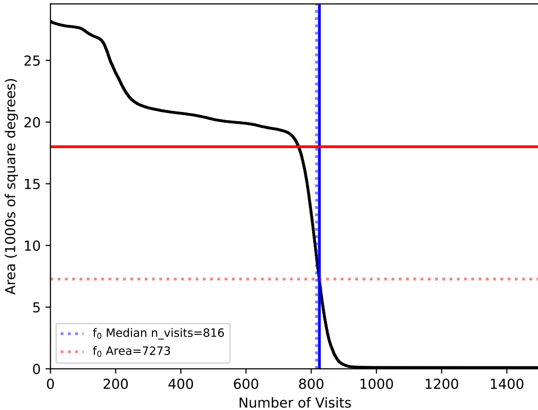
too_elab_heavy_r64_d3_griz_v3.4_10yrs All sky: f0
