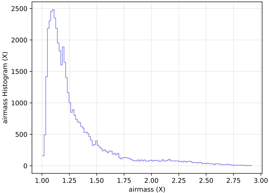
too_elab_heavy_r64_d3_griz_v3.4_10yrs Yr 1 z band: airmass Histogram
