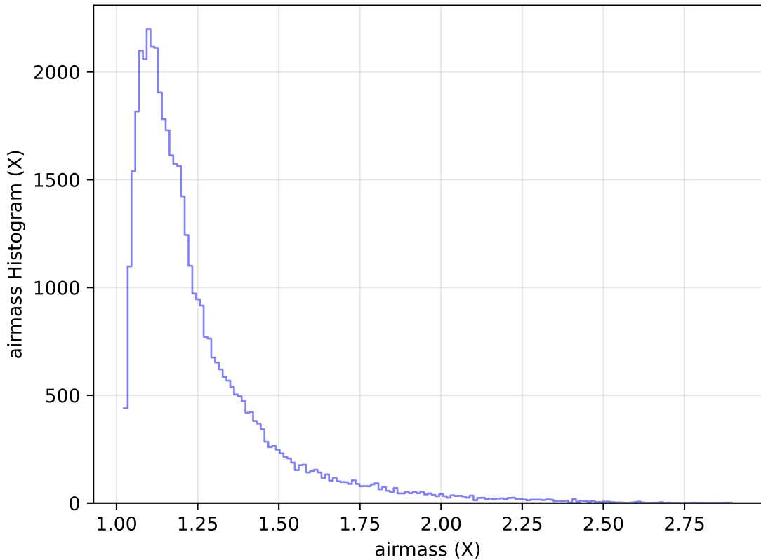
too_elab_heavy_r64_d3_griz_v3.4_10yrs Yr 1 y band: airmass Histogram
