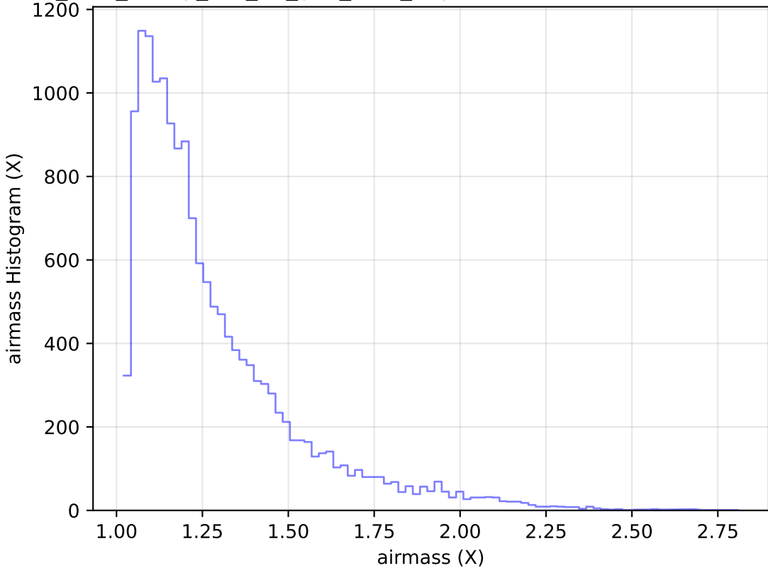
too_elab_heavy_r64_d3_griz_v3.4_10yrs Yr 1 u band: airmass Histogram
