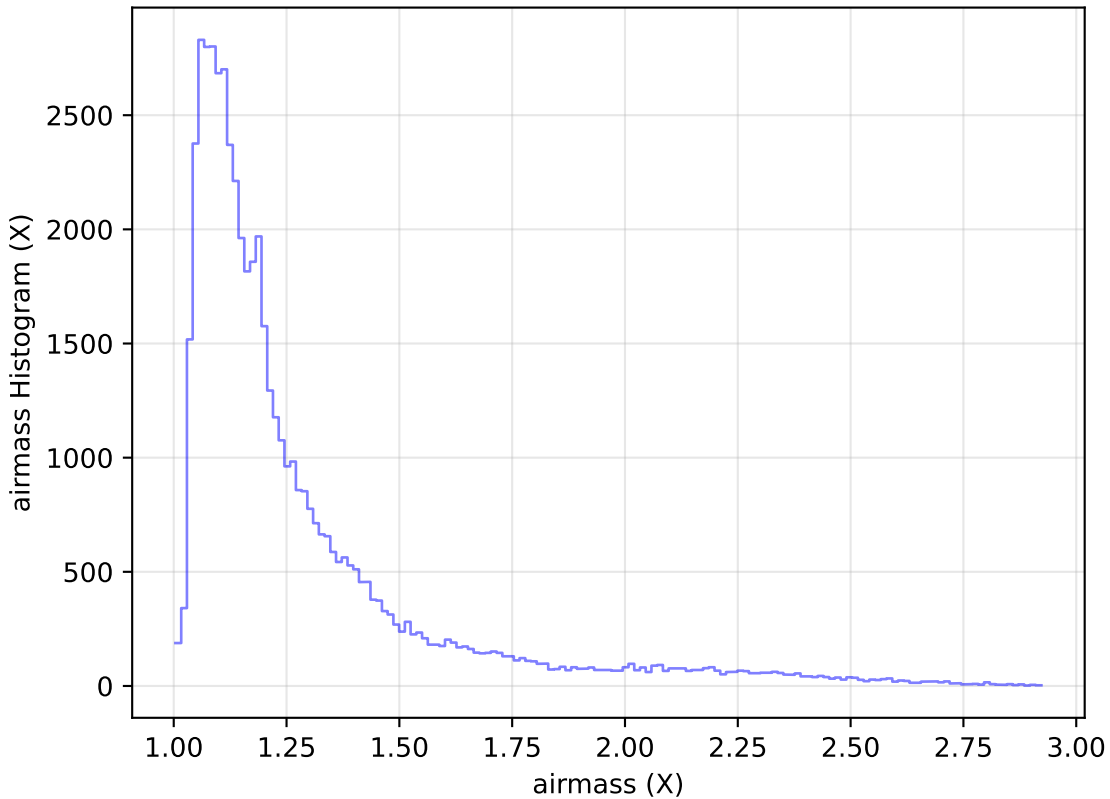
too_elab_heavy_r64_d3_griz_v3.4_10yrs Yr 1 i band: airmass Histogram
