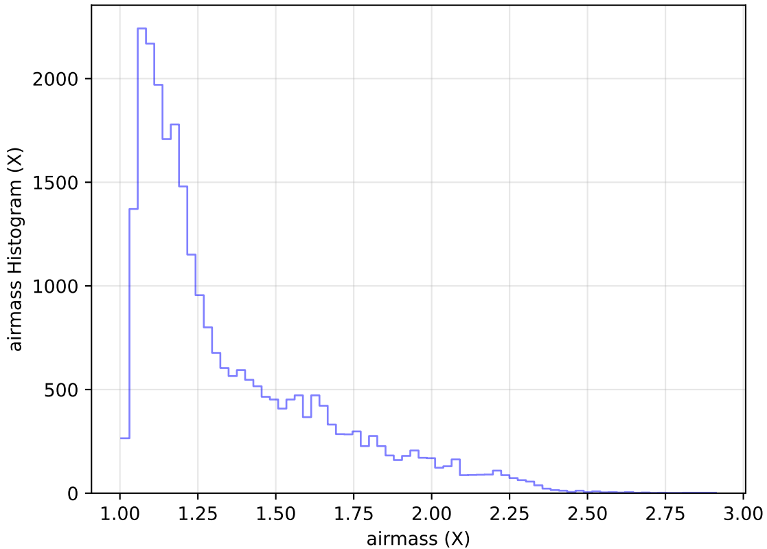
too_elab_heavy_r64_d3_griz_v3.4_10yrs Yr 1 g band: airmass Histogram
