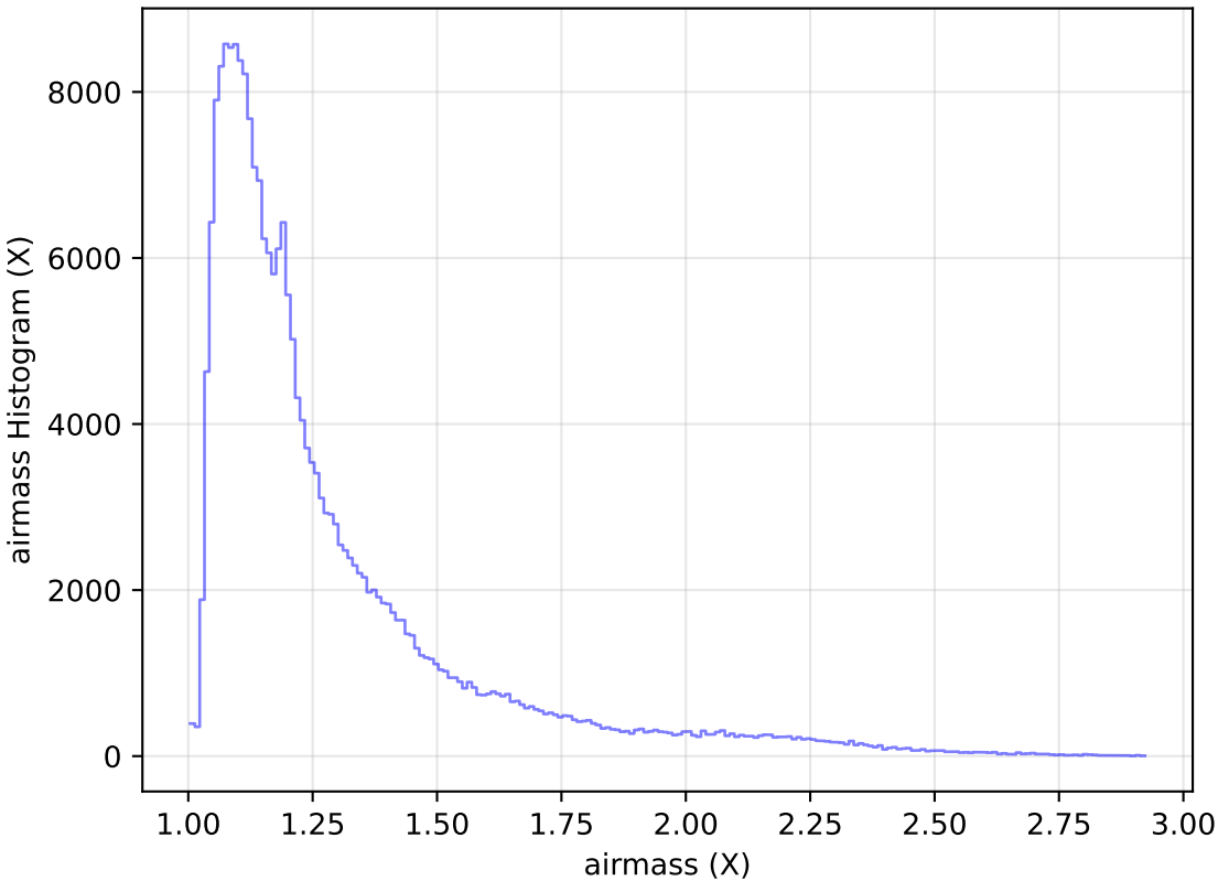
too_elab_heavy_r64_d3_griz_v3.4_10yrs Yr 1 all bands: airmass Histogram
