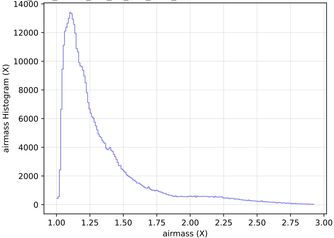
too_elab_heavy_r64_d3_griz_v3.4_10yrs WFD z band: airmass Histogram
