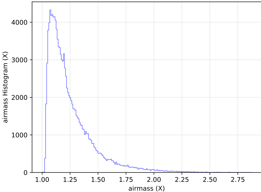
too_elab_heavy_r64_d3_griz_v3.4_10yrs WFD u band: airmass Histogram
