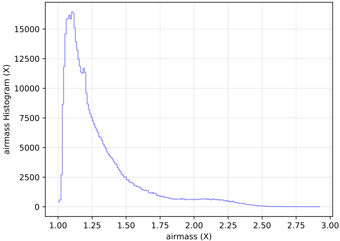
too_elab_heavy_r64_d3_griz_v3.4_10yrs WFD r band: airmass Histogram
