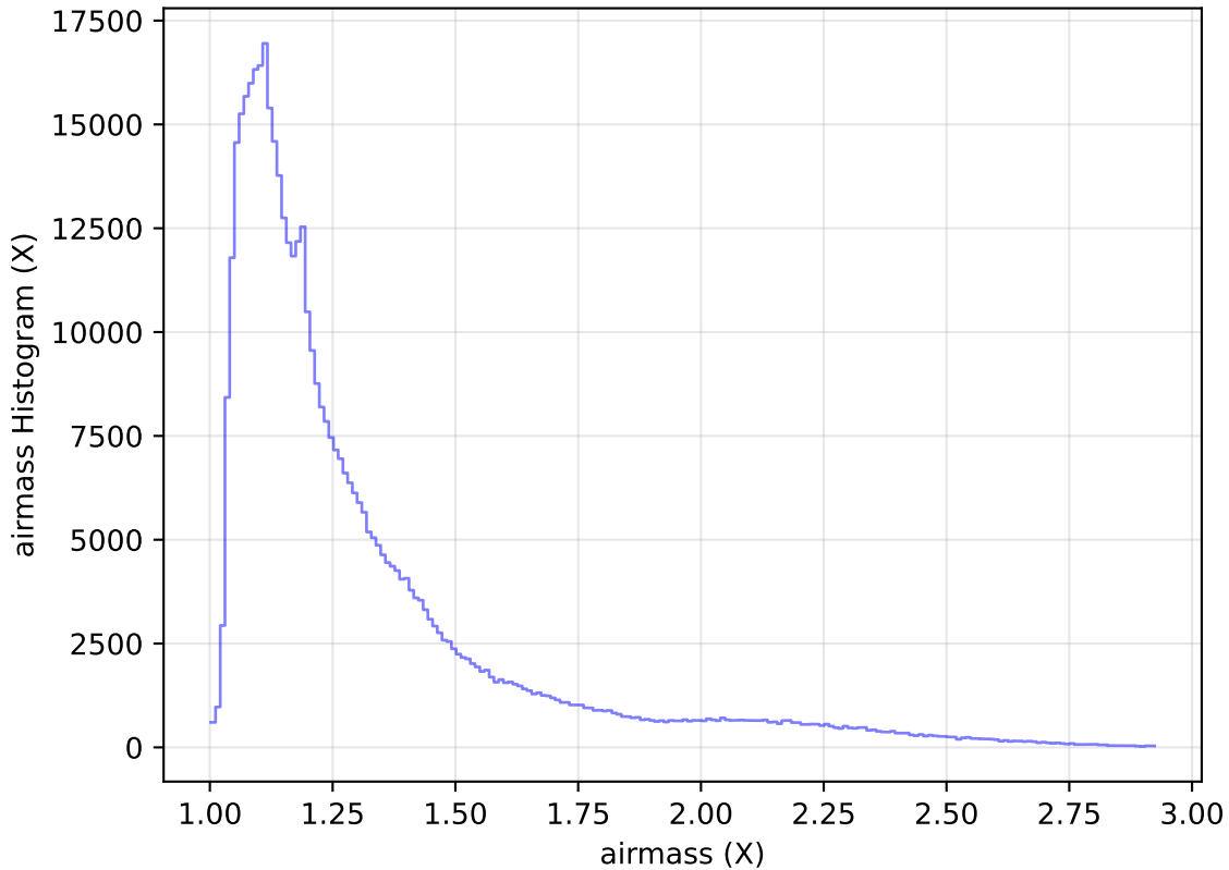
too_elab_heavy_r64_d3_griz_v3.4_10yrs WFD i band: airmass Histogram
