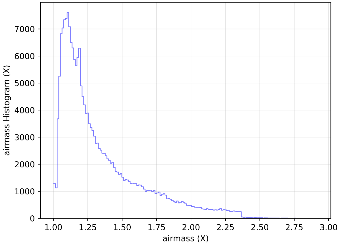
too_elab_heavy_r64_d3_griz_v3.4_10yrs WFD g band: airmass Histogram
