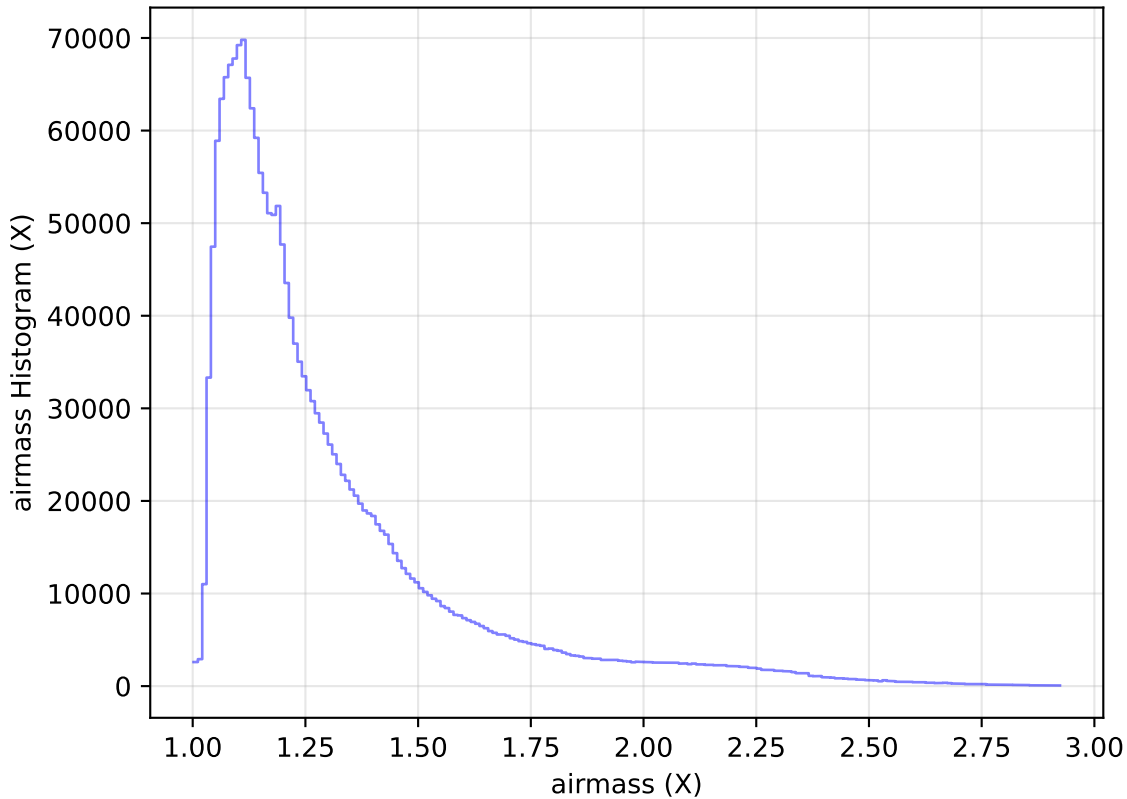
too_elab_heavy_r64_d3_griz_v3.4_10yrs WFD all bands: airmass Histogram
