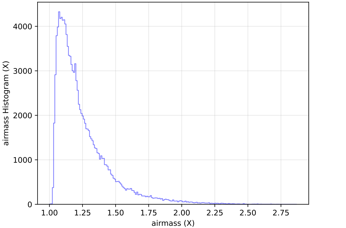
too_elab_heavy_r64_d3_griz_v3.4_10yrs All sky u band: airmass Histogram
