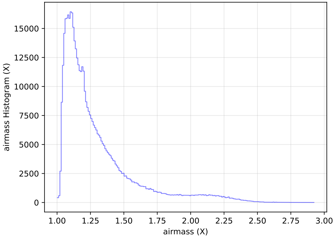
too_elab_heavy_r64_d3_griz_v3.4_10yrs All sky r band: airmass Histogram
