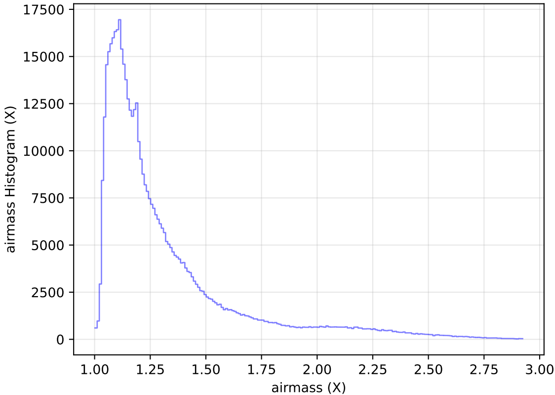
too_elab_heavy_r64_d3_griz_v3.4_10yrs All sky i band: airmass Histogram
