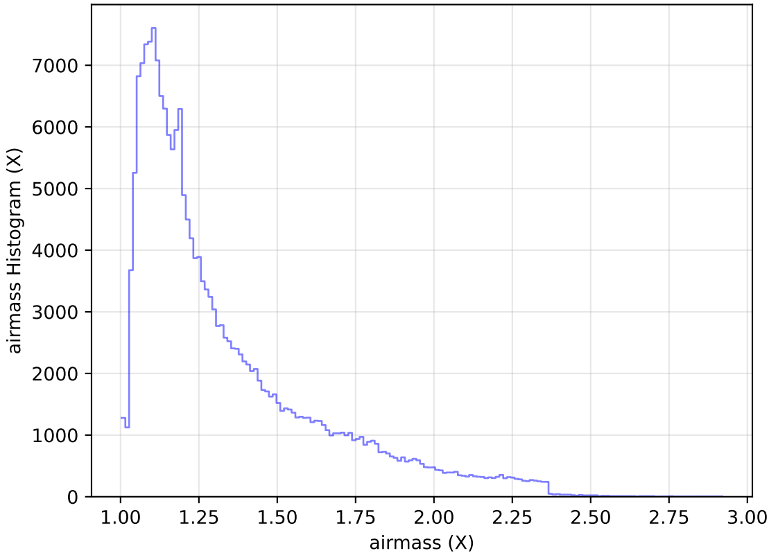
too_elab_heavy_r64_d3_griz_v3.4_10yrs All sky g band: airmass Histogram
