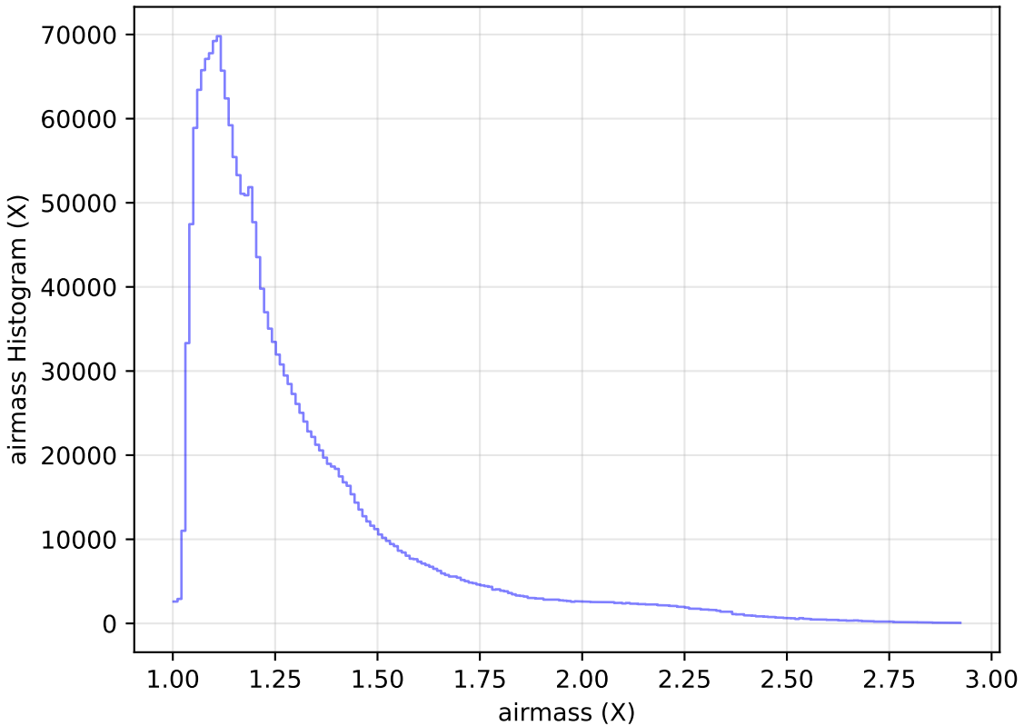
too_elab_heavy_r64_d3_griz_v3.4_10yrs All sky all bands: airmass Histogram
