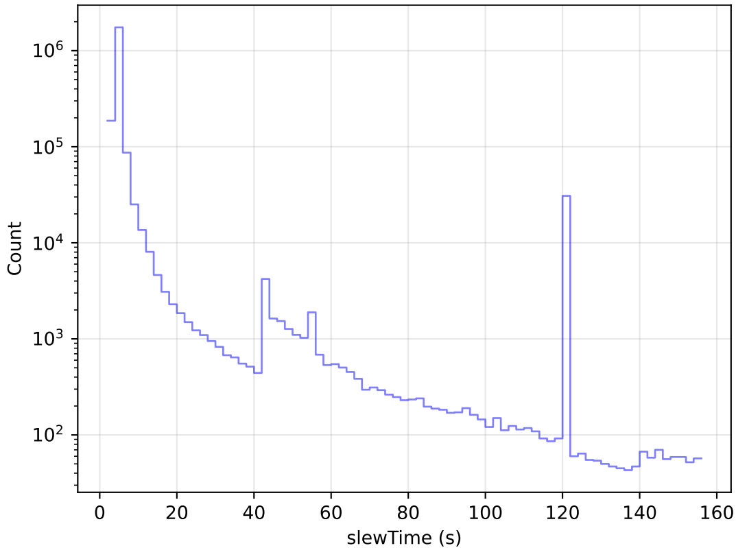
too_elab_heavy_r64_d3_griz_v3.4_10yrs All visits: Slew Time Histogram
