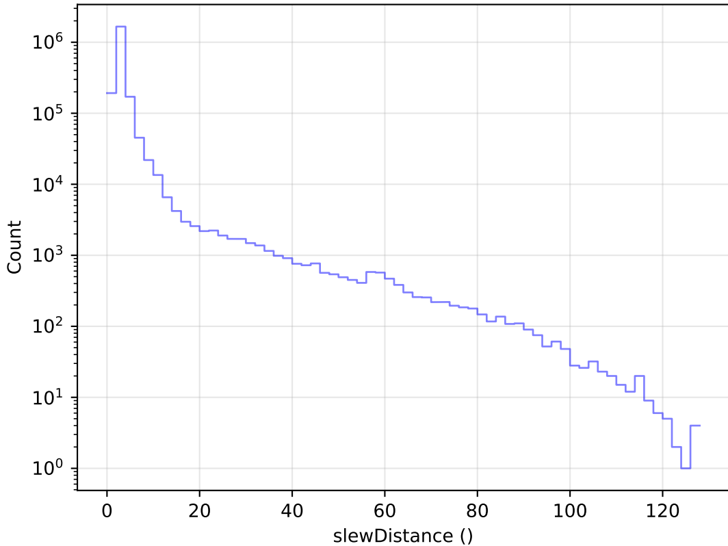
too_elab_heavy_r64_d3_griz_v3.4_10yrs All visits: Slew Distance Histogram
