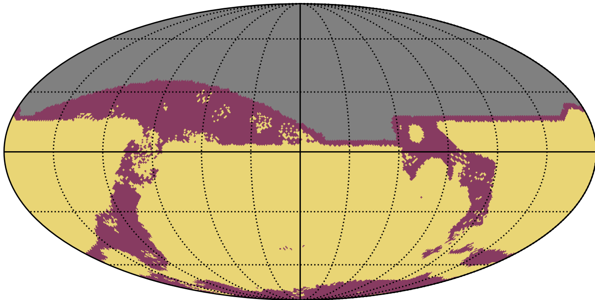
too_elab_heavy_r64_d3_griz_v3.4_10yrs All sky: RapidRevisits
