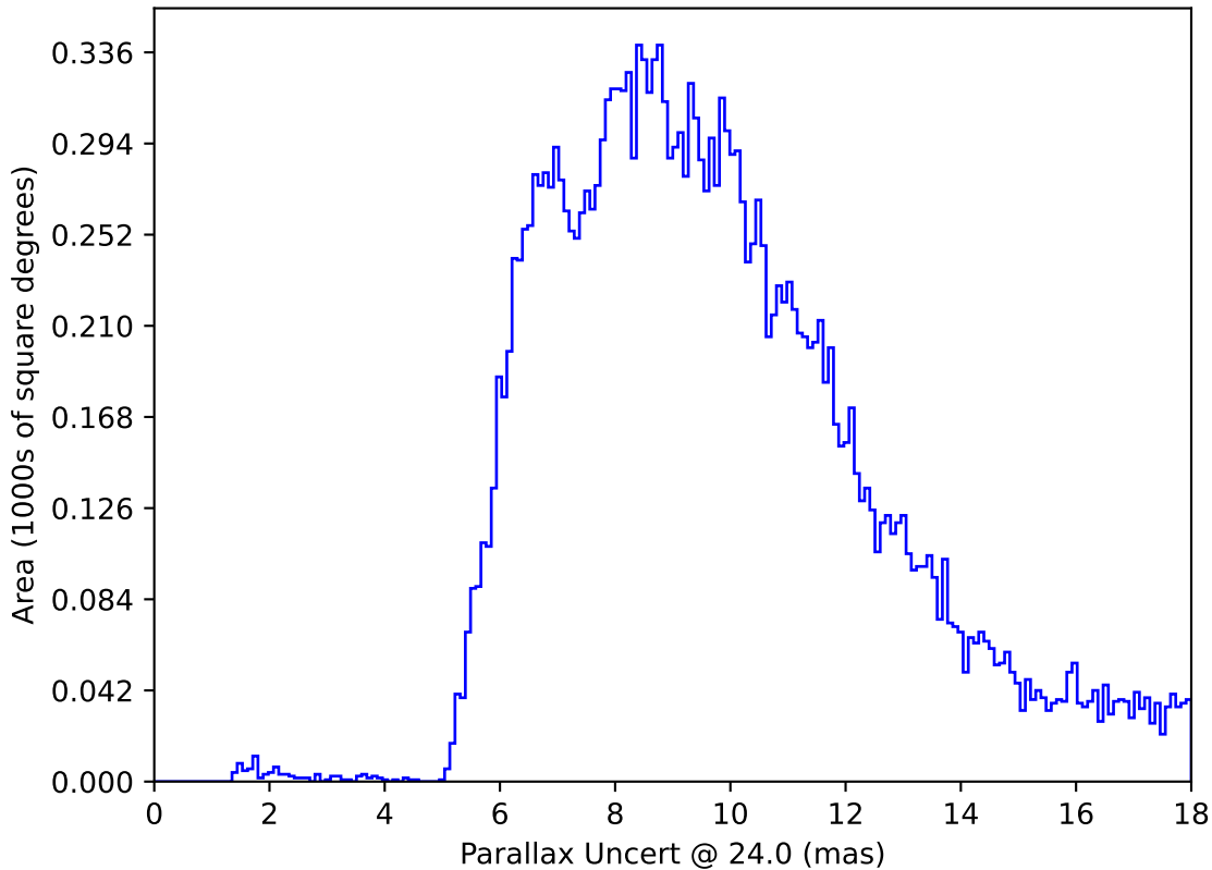
too_elab_heavy_r64_d3_griz_v3.4_10yrs All sky: Parallax Uncert @ 24.0
