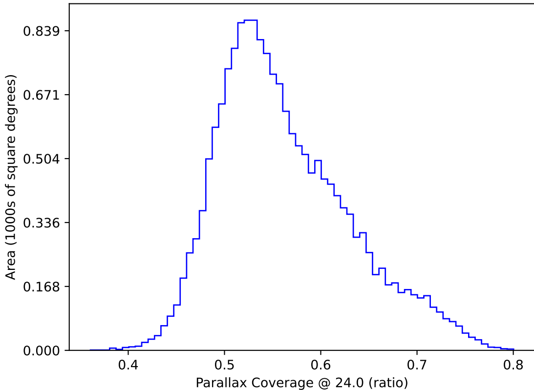
too_elab_heavy_r64_d3_griz_v3.4_10yrs WFD: Parallax Coverage @ 24.0
