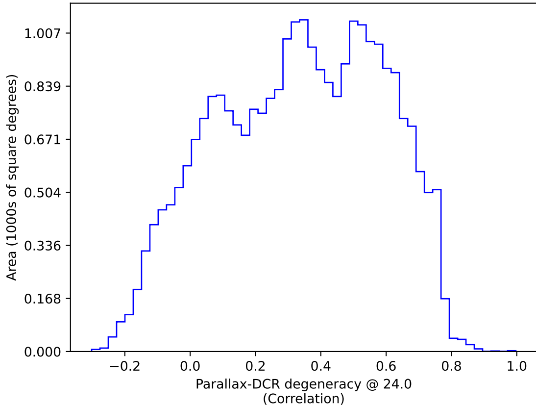
too_elab_heavy_r64_d3_griz_v3.4_10yrs All sky: Parallax-DCR degeneracy @ 24.0
