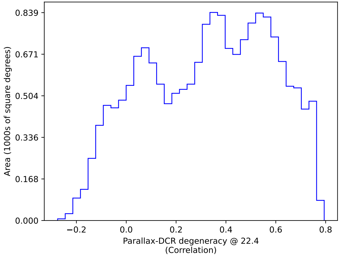
too_elab_heavy_r64_d3_griz_v3.4_10yrs WFD: Parallax-DCR degeneracy @ 22.4
