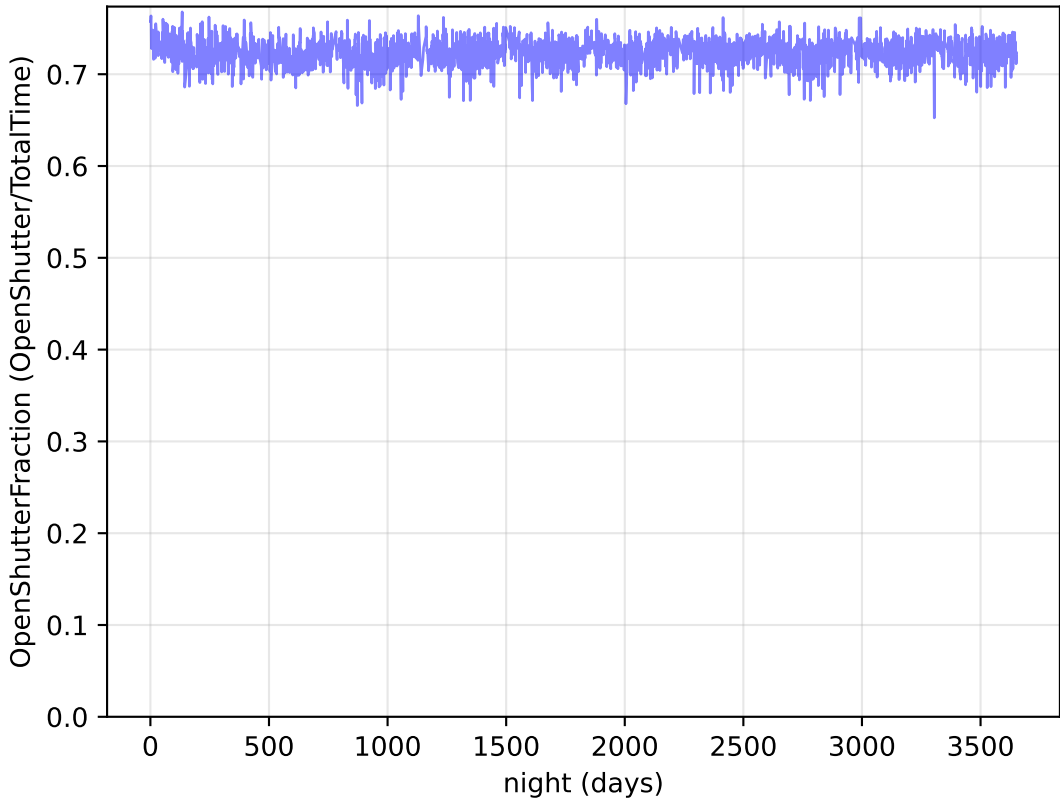
too_elab_heavy_r64_d3_griz_v3.4_10yrs Per night: OpenShutterFraction
