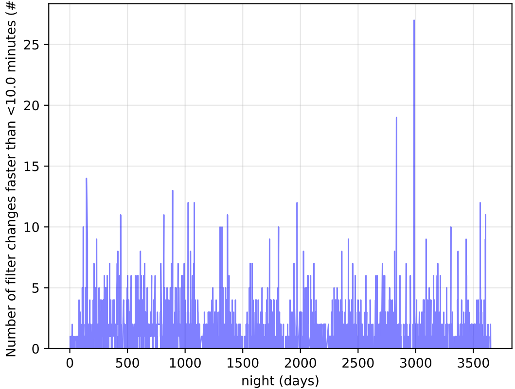
too_elab_heavy_r64_d3_griz_v3.4_10yrs Per Night: Number of filter changes faster than <10.0 minutes
