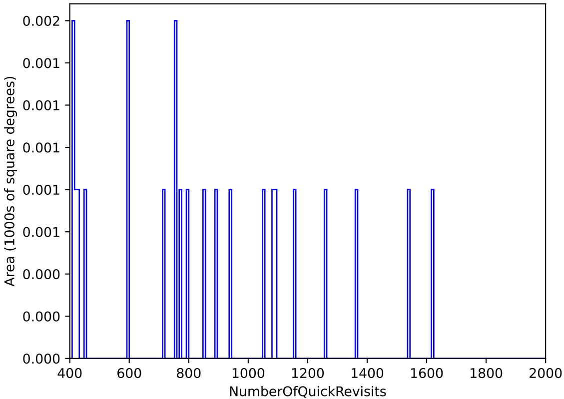
too_elab_heavy_r64_d3_griz_v3.4_10yrs WFD: NumberOfQuickRevisits
