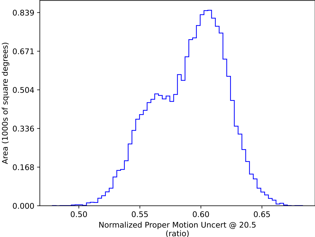
too_elab_heavy_r64_d3_griz_v3.4_10yrs WFD: Normalized Proper Motion Uncert @ 20.5
