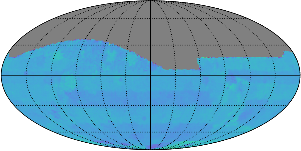
too_elab_heavy_r64_d3_griz_v3.4_10yrs All sky: Normalized Proper Motion Uncert @ 20.5
