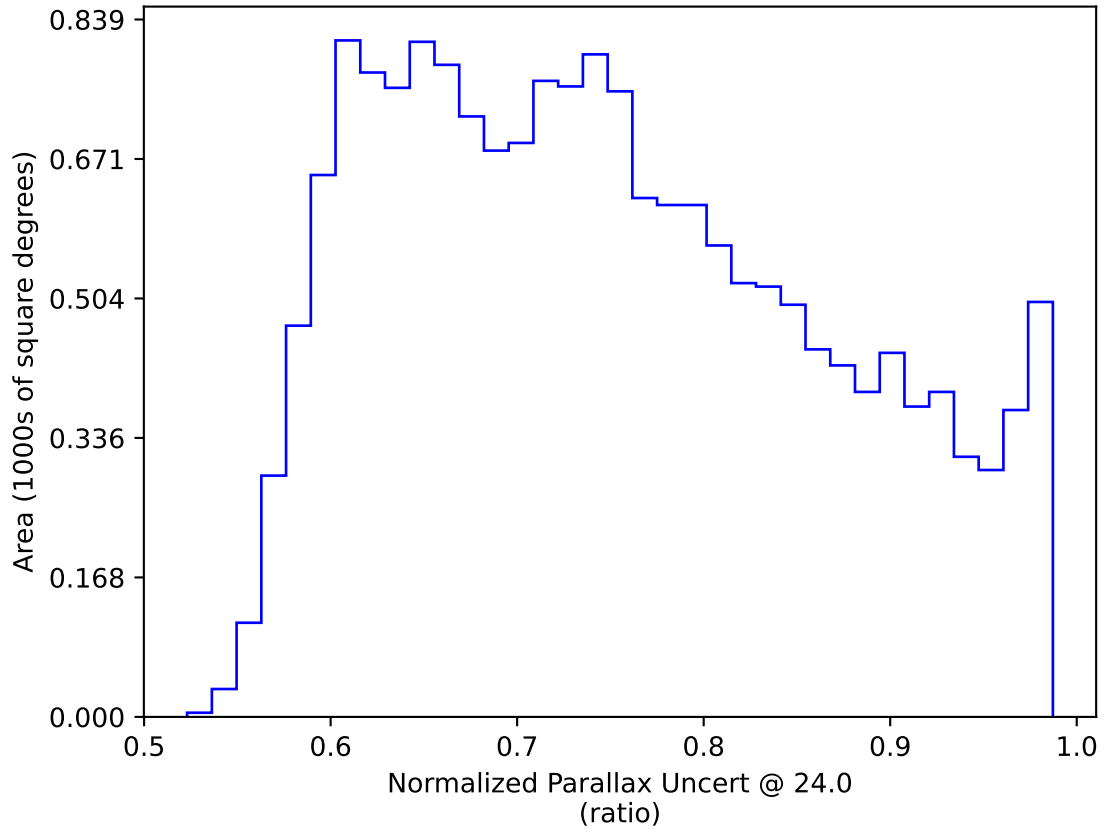
too_elab_heavy_r64_d3_griz_v3.4_10yrs WFD: Normalized Parallax Uncert @ 24.0
