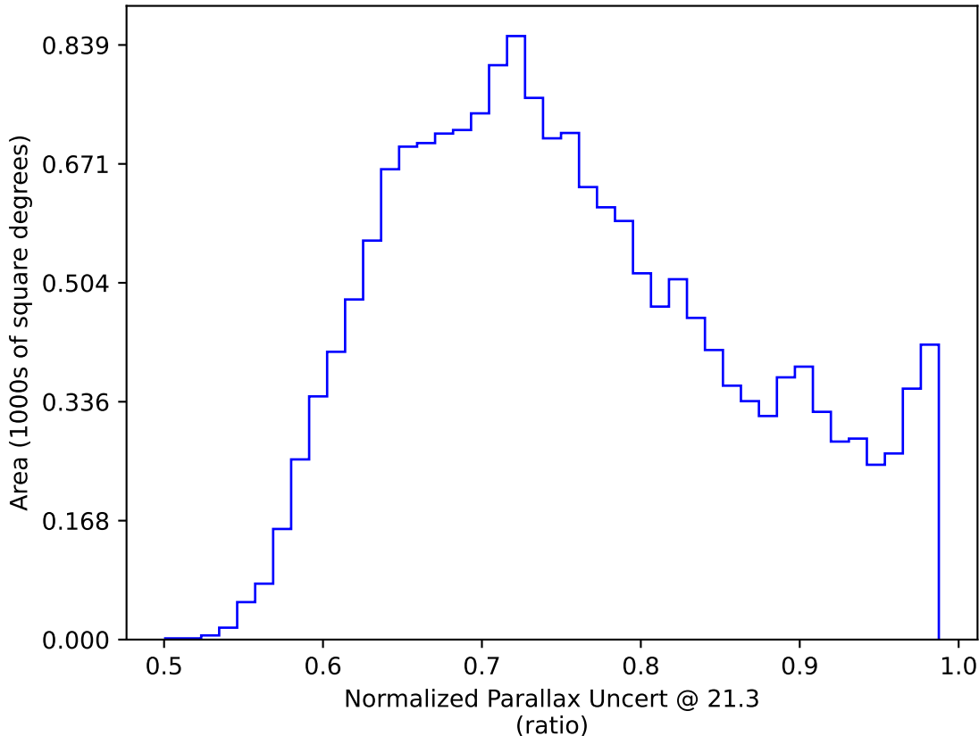
too_elab_heavy_r64_d3_griz_v3.4_10yrs WFD y band only: Normalized Parallax Uncert @ 21.3
