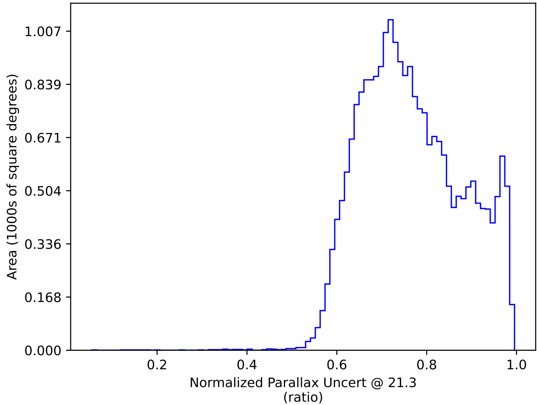
too_elab_heavy_r64_d3_griz_v3.4_10yrs All sky y band only: Normalized Parallax Uncert @ 21.3
