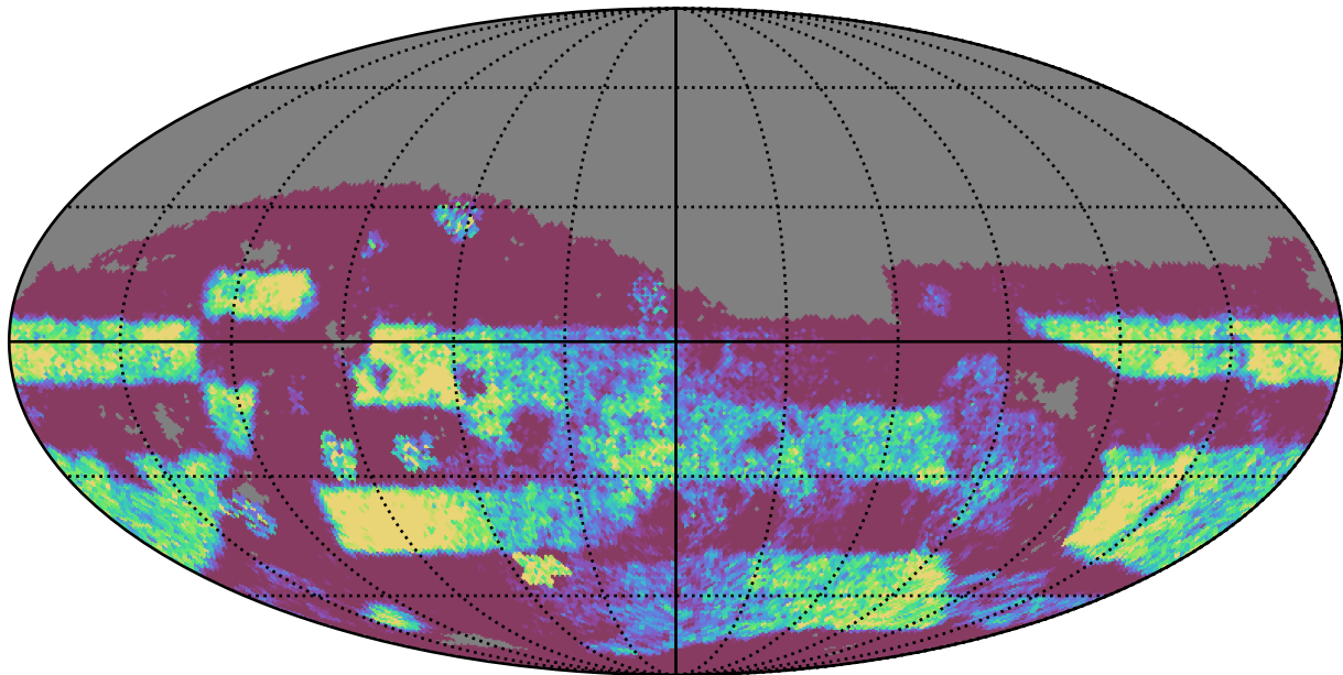
too_elab_heavy_r64_d3_griz_v3.4_10yrs Yr 3-4 z band: NVisits
