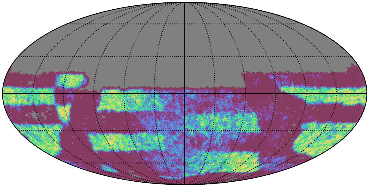
too_elab_heavy_r64_d3_griz_v3.4_10yrs Yr 3-4 y band: NVisits
