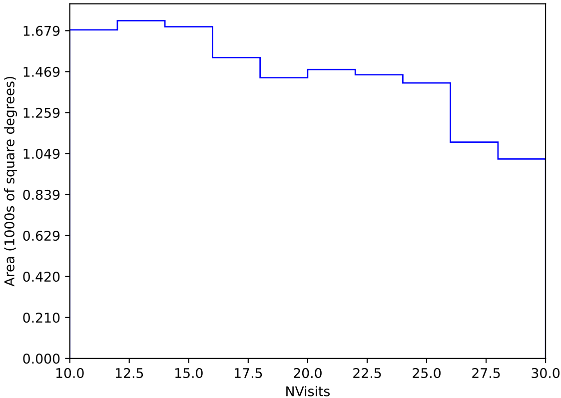
too_elab_heavy_r64_d3_griz_v3.4_10yrs Yr 3-4 y band: NVisits
