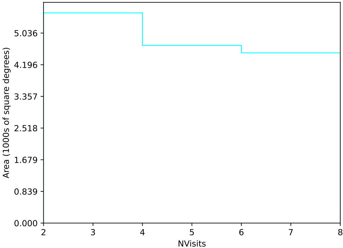
too_elab_heavy_r64_d3_griz_v3.4_10yrs Yr 3-4 u band: NVisits
