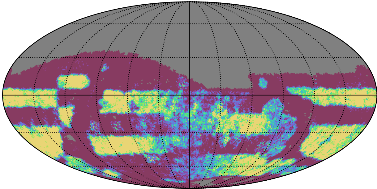
too_elab_heavy_r64_d3_griz_v3.4_10yrs Yr 3-4 r band: NVisits
